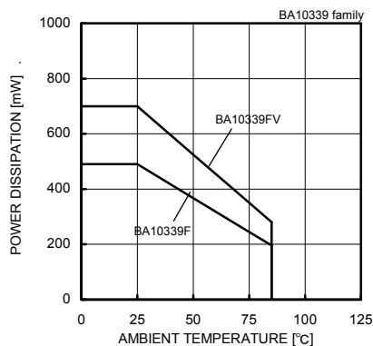
Fig. 21 Derating Curve
