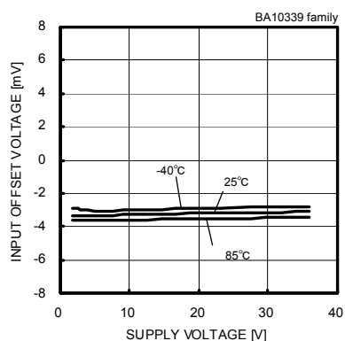
Fig. 28 Input Offset Voltage - Supply Voltage
